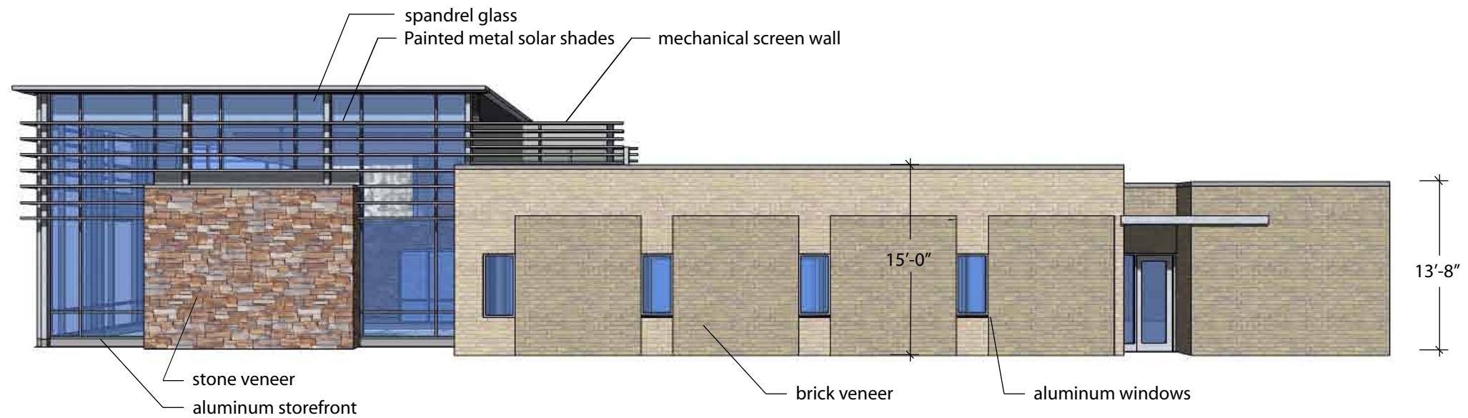
SOUTH ELEVATION
