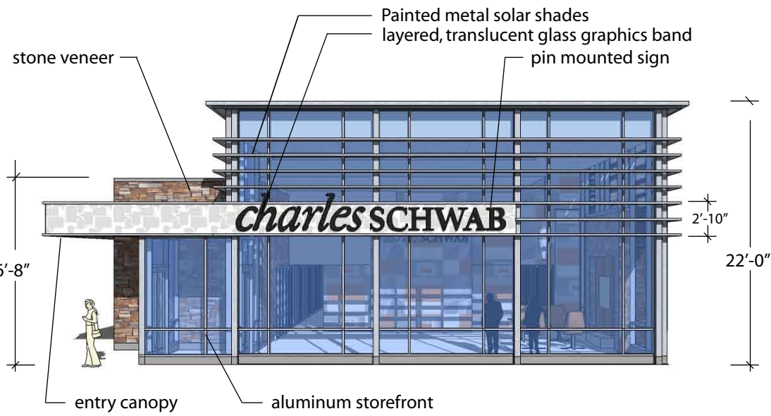
WEST ELEVATION
